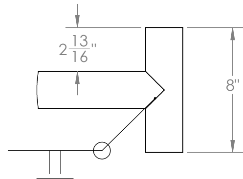
DETAIL C SCALE 1 : 6
