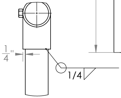
DETAIL D SCALE 1 : 6
